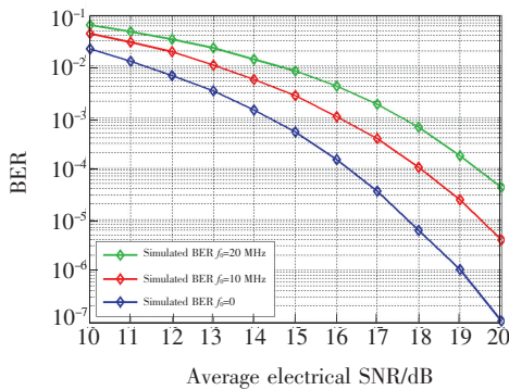
图 4 具有不同频偏的联合校正系统仿真误码率 Fig. 4 Simulated BERs of the system using joint algorithm with different frequency offset
