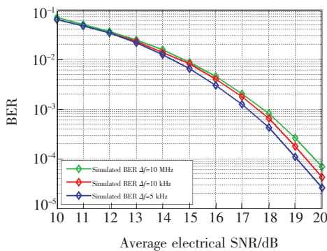
图 5 具有不同联合线宽的联合校正系统仿真误码率 Fig. 5 Simulated BERs of the system using joint algorithm with different linewidth
